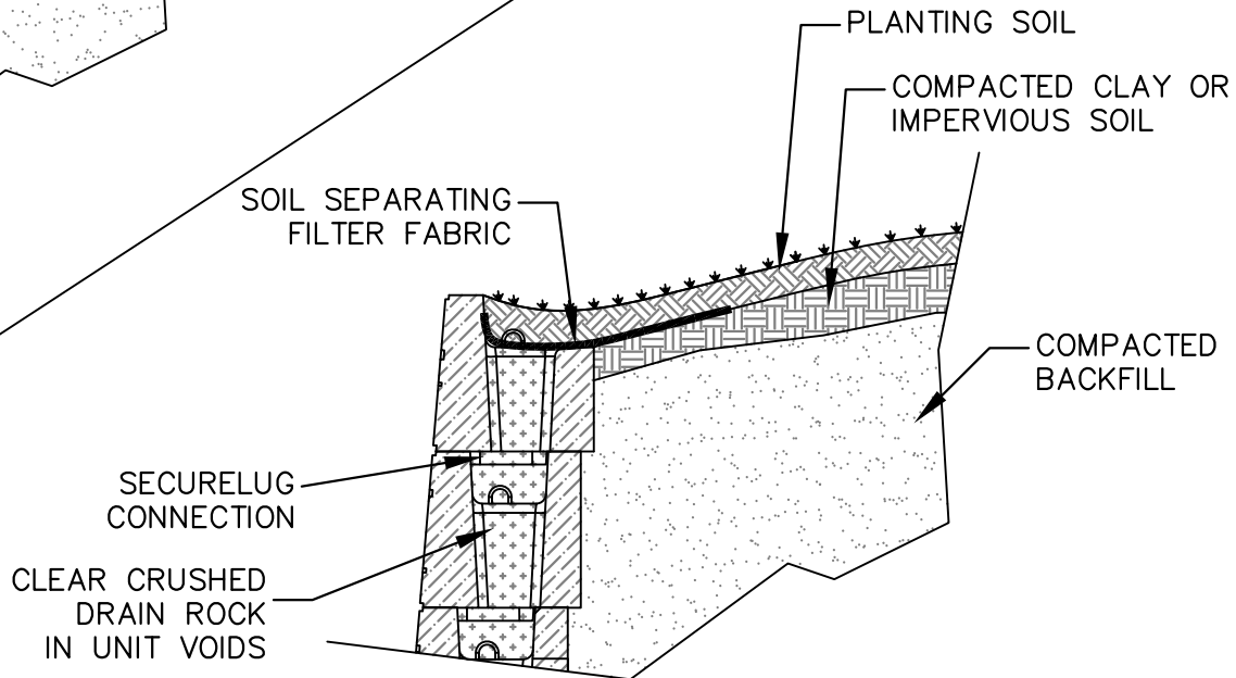
COMPACTED CLAY OR IMPERVIOUS SOIL SWALE SECTION
