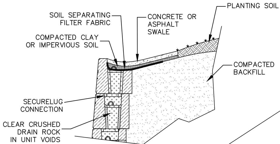
CONCRETE OR ASPHALT SWALE SECTION
