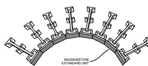
INSIDE CURVE
