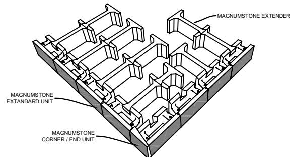
OUTSIDE CORNER
