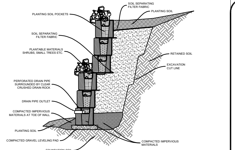
6.0 FT PLANTABLE WALL
