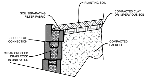
CLAY / IMPERVIOUS SWALE
