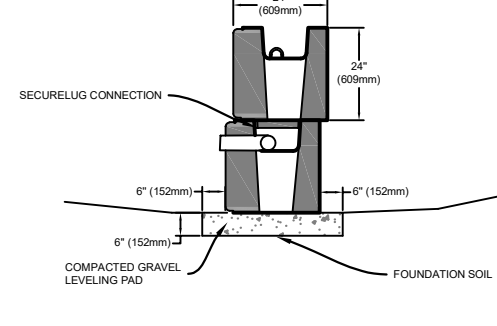
LEVELING PAD
