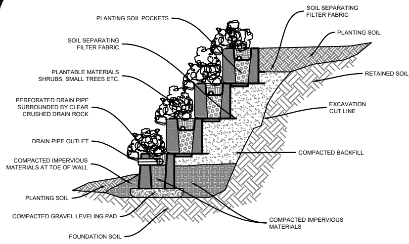
2.0 FT PLANTABLE WALL
