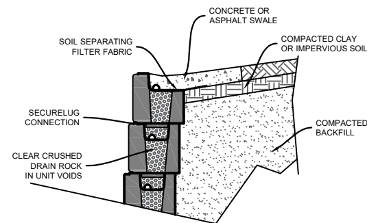
CONCRETE / ASPHALT SWALE
