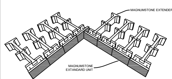
INSIDE CORNER
