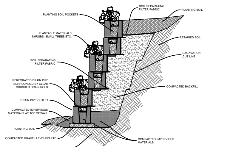
4.0 FT PLANTABLE WALL
