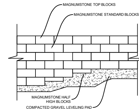
BASE STEP UP
