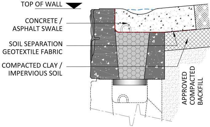
CONCRETE TOP SWALE
