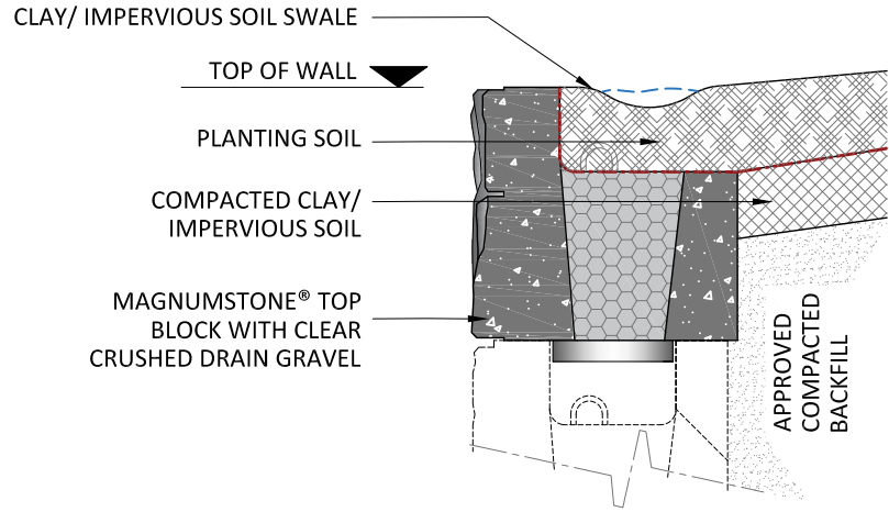
IMPERVIOUS MATERIAL TOP SWALE
