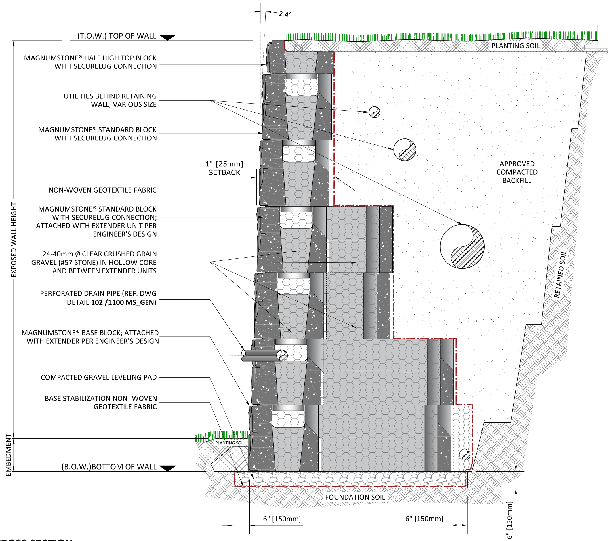
01 WALL CROSS SECTION SCALE 1 : 20
