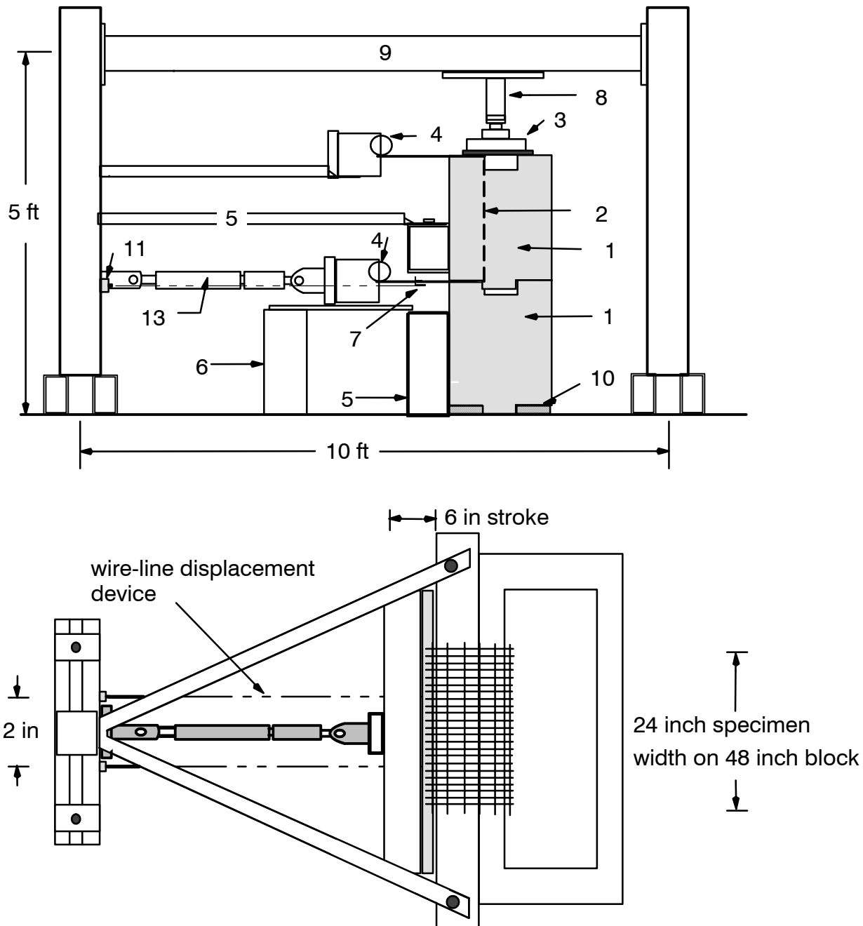
Figure 1: Schematic of connection test apparatus showing MagnumStone block units and Tensar UX1600 geogrid
