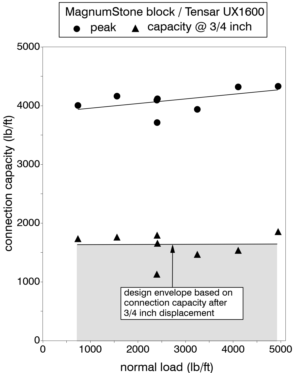
Figure 5: Preliminary design capacity envelope for MagnumStone block / Tensar UX1600 combination
