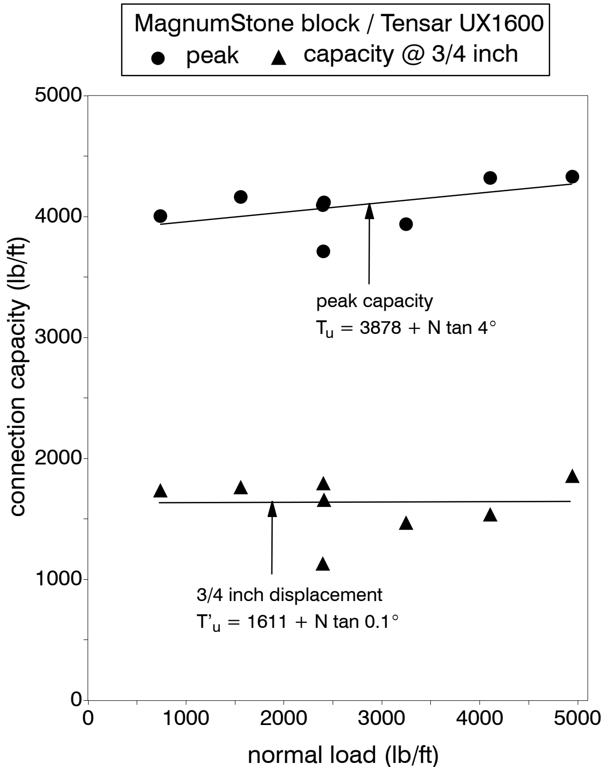
Figure 4: MagnumStone block / Tensar UX1600 connection capacity test results
