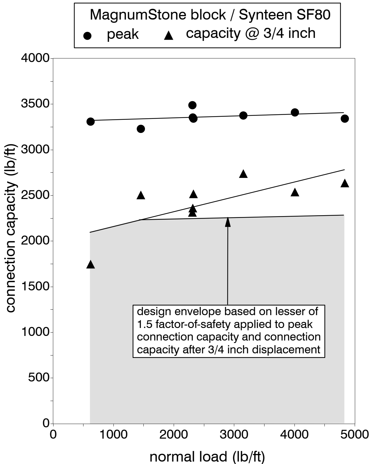
Figure 5: Preliminary design capacity envelope for MagnumStone block / Synteen SF80 geogrid combination
