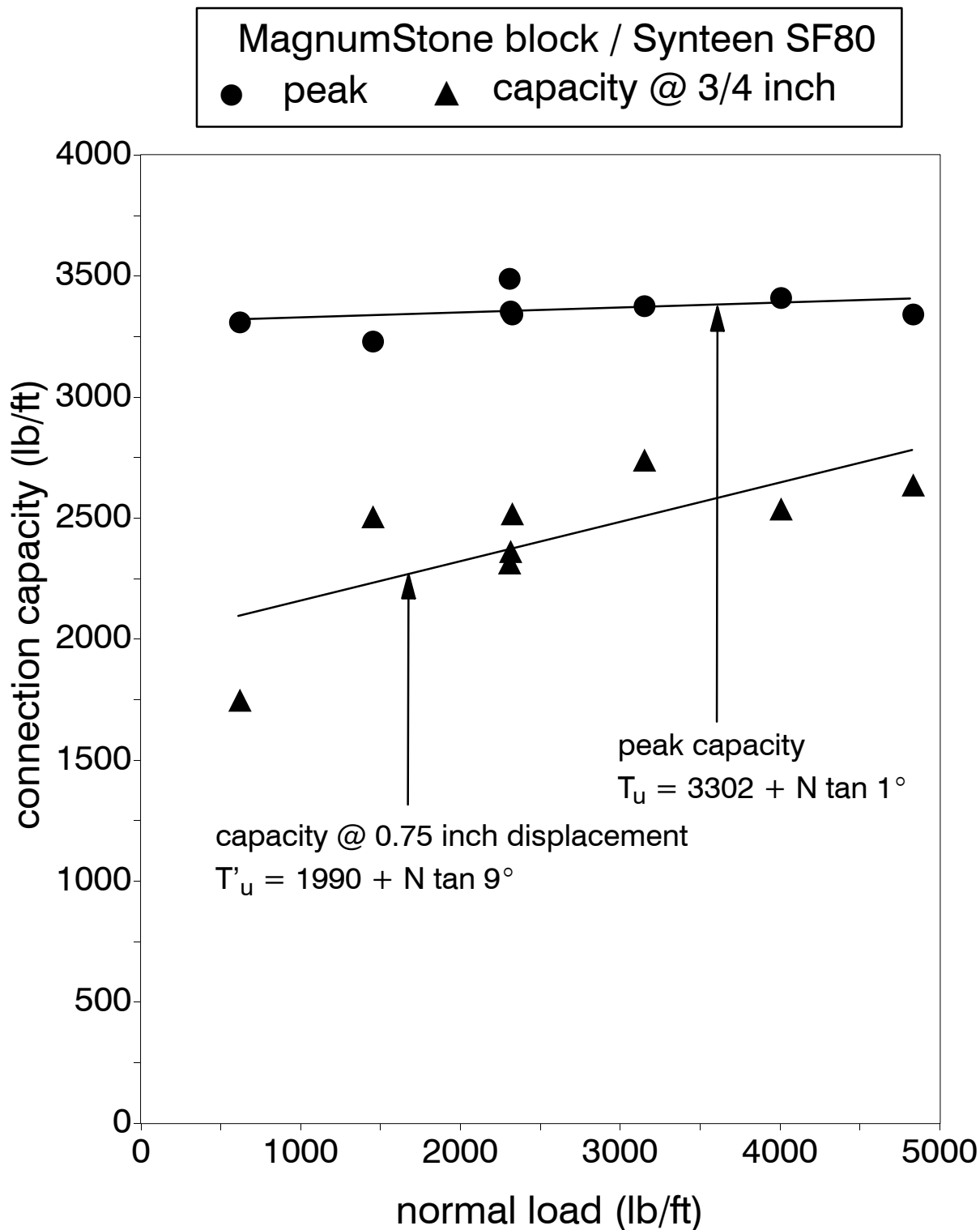
Figure 4: MagnumStone block / Synteen SF80 connection capacity test results
