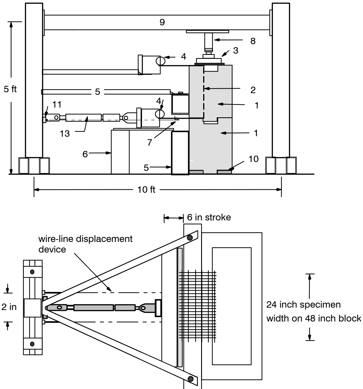
Figure 1: Schematic of connection test apparatus showing MagnumStone block units and Synteen SF80 geogrid
