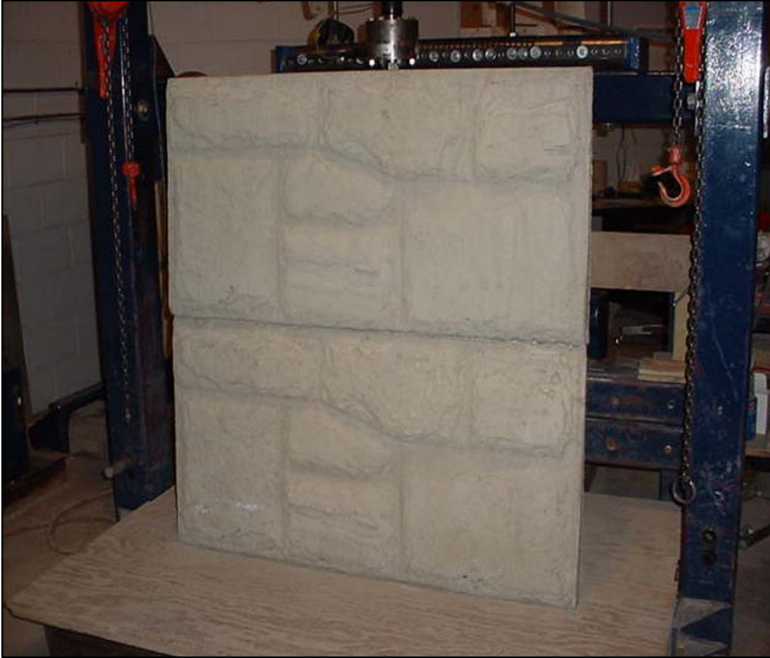
Figure 3: Photograph of the MagnumStone blocks in the connection frame
