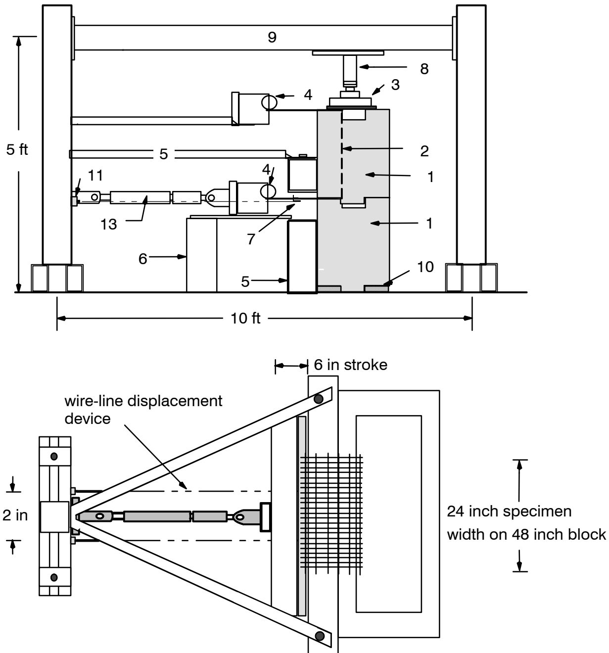
Figure 1: Schematic of connection test apparatus showing MagnumStone block units and Raugrid 6X3N geogrid
