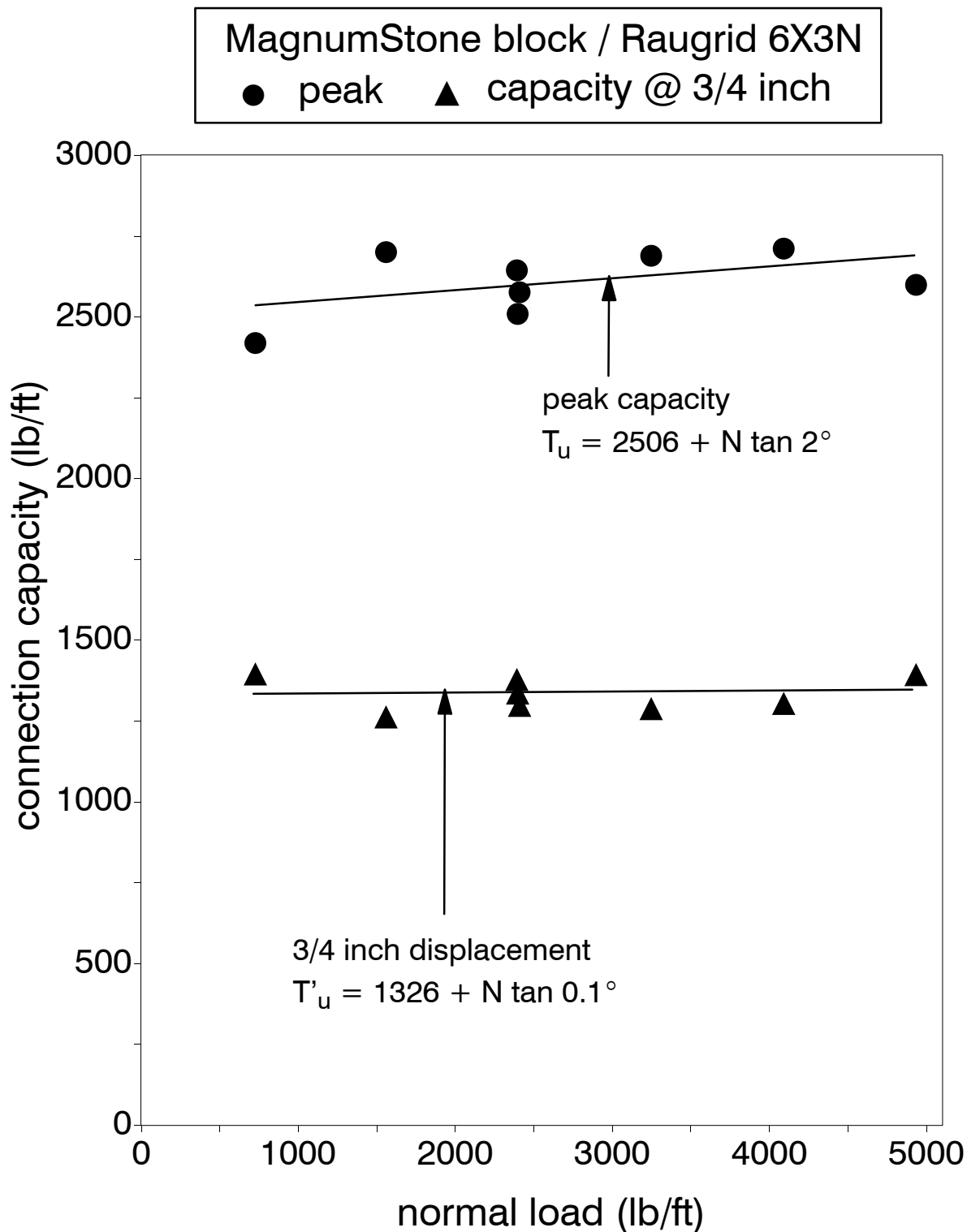
Figure 4: MagnumStone block / Raugrid 6X3N connection capacity test results
