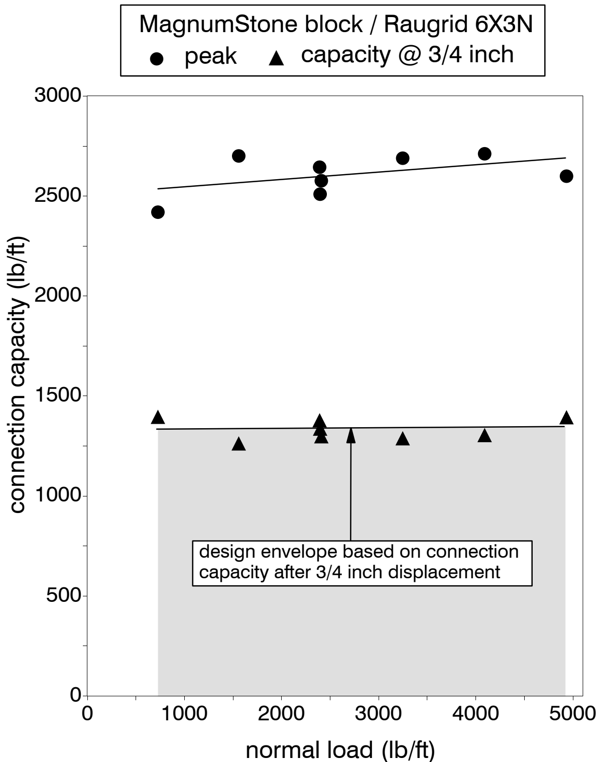
Figure 5: Preliminary design capacity envelope for MagnumStone block / Raugrid 6X3N combination
