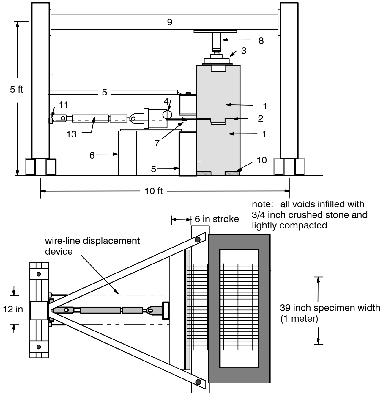
Figure 1: Schematic of connection test apparatus showing MagnumStone block units (frictional connection configuration) and Miragrid 5XT geogrid
