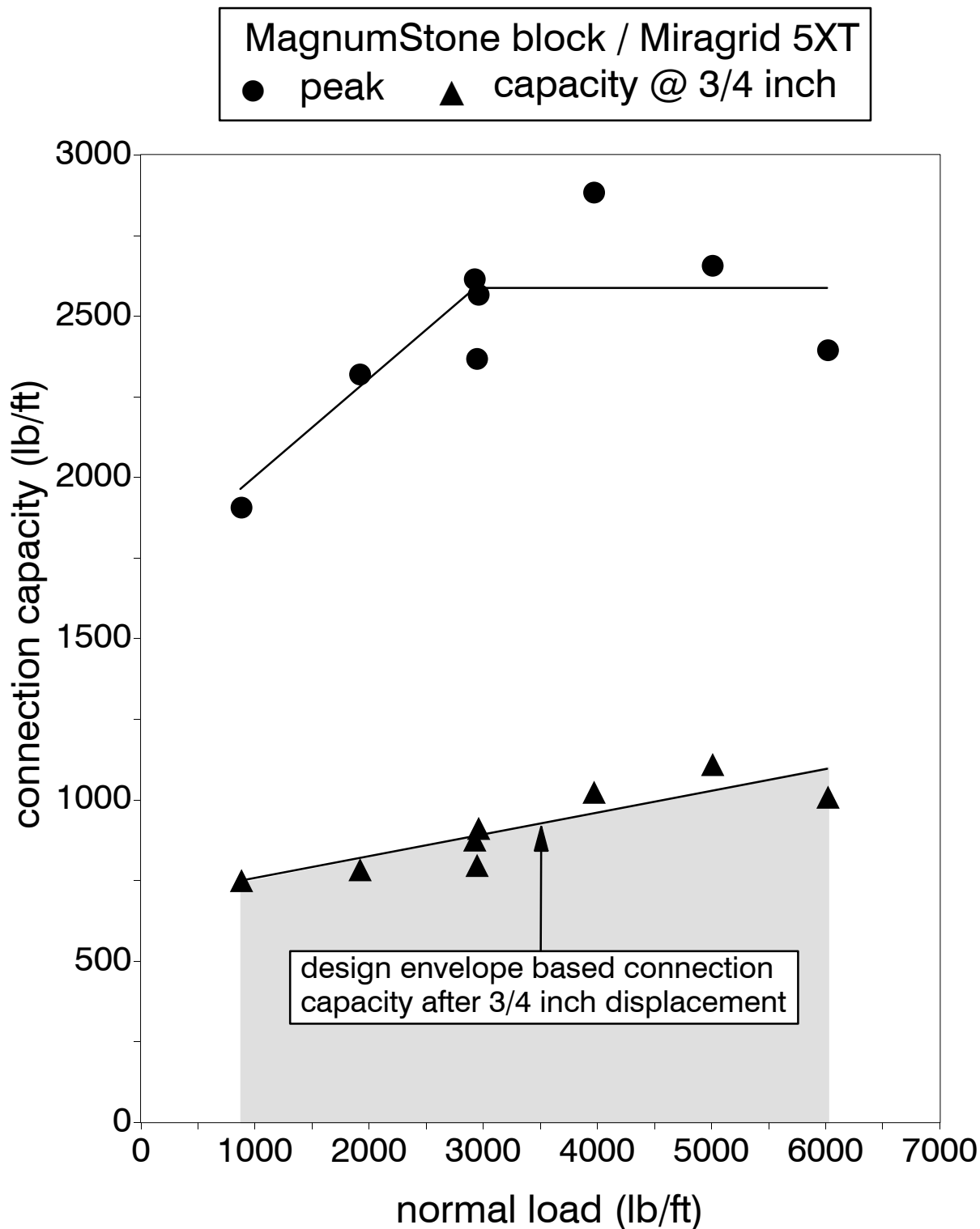
Figure 5: Preliminary design capacity envelope for MagnumStone block (frictional) / Miragrid 5XT geogrid combination
