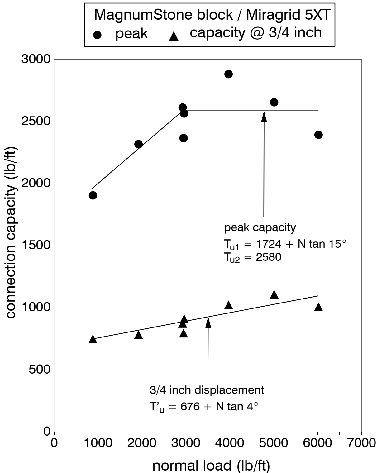
Figure 4: MagnumStone block (frictional) / Miragrid 5XT connection capacity test results
