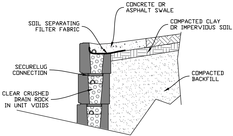
CONCRETE / ASPHALT SWALE
