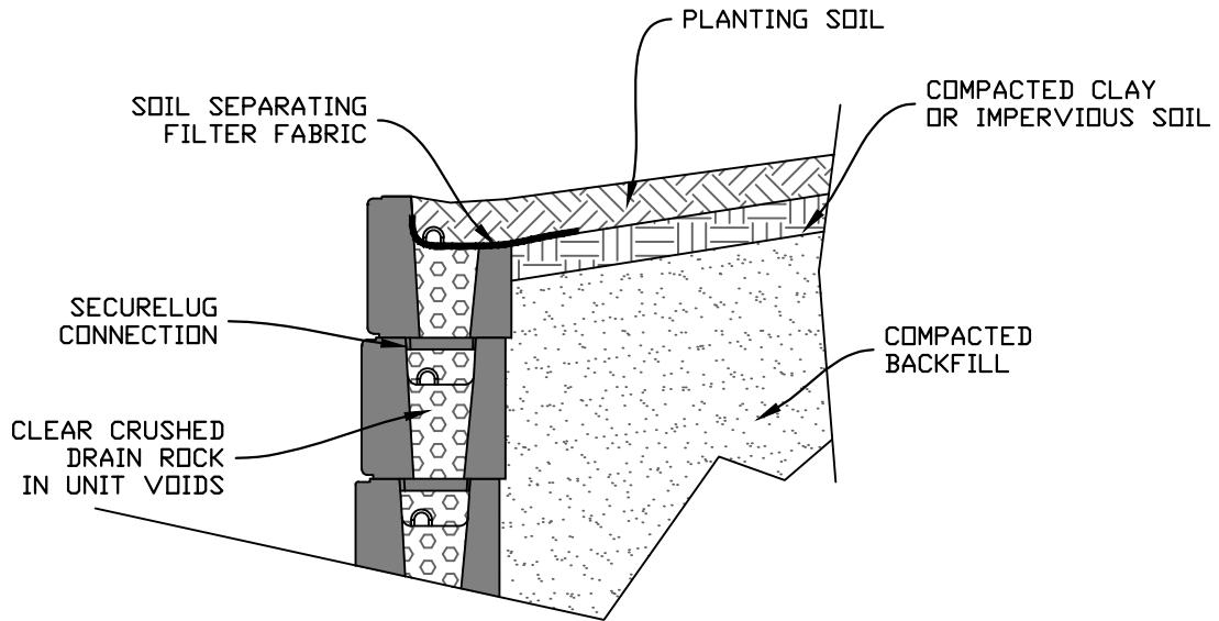
COMPACTED CLAY / IMPERVIOUS SOIL SWALE
